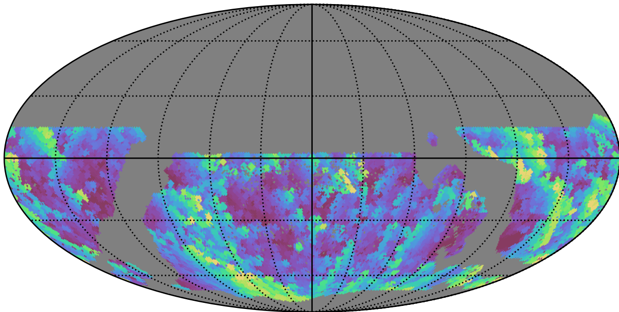
mw_roll_bulge_v3.3_10yrs WFD u band: Max airmass
