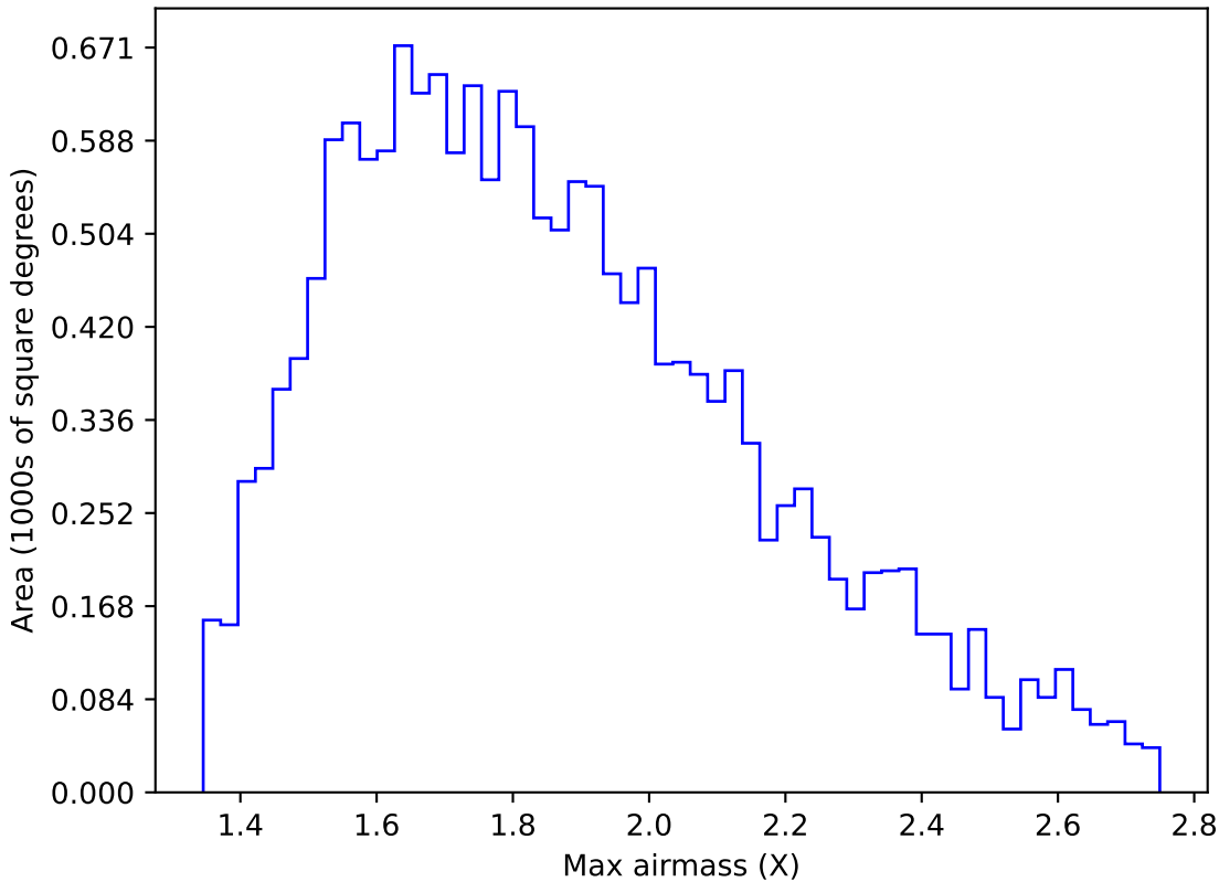
mw_roll_bulge_v3.3_10yrs WFD u band: Max airmass
