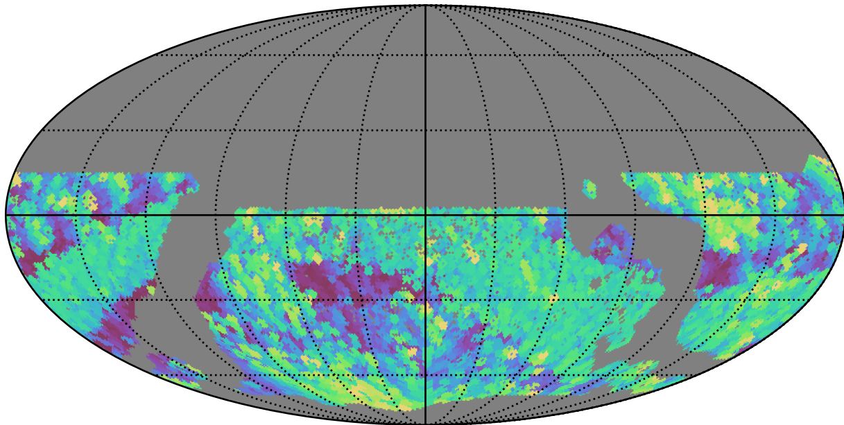
mw_roll_bulge_v3.3_10yrs WFD r band: Max airmass
