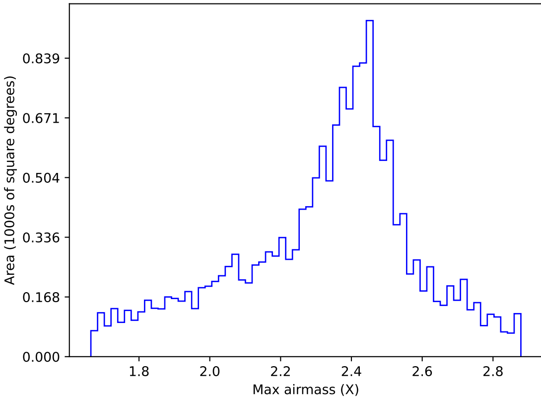
mw_roll_bulge_v3.3_10yrs WFD r band: Max airmass
