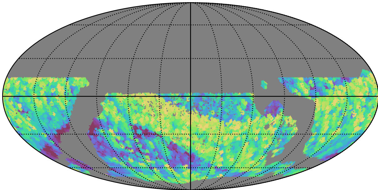
mw_roll_bulge_v3.3_10yrs WFD i band: Max airmass
