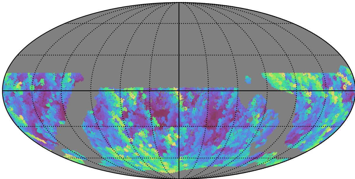
mw_roll_bulge_v3.3_10yrs WFD g band: Max airmass
