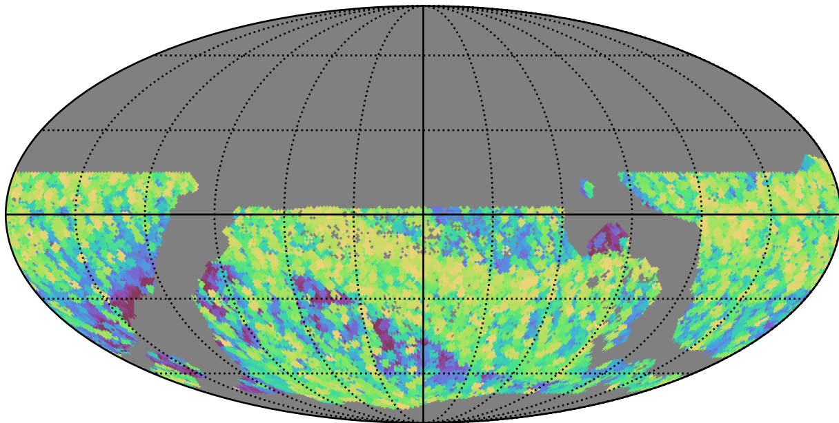
mw_roll_bulge_v3.3_10yrs WFD all bands: Max airmass
