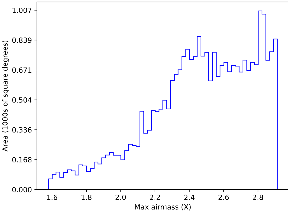
mw_roll_bulge_v3.3_10yrs All sky z band: Max airmass
