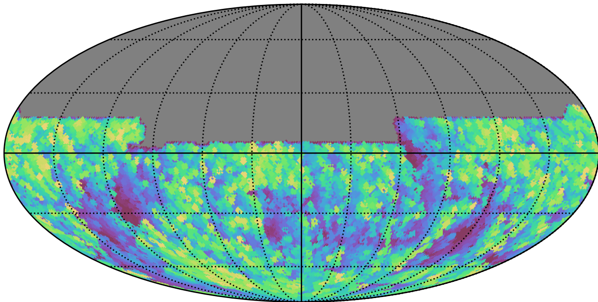
mw_roll_bulge_v3.3_10yrs All sky y band: Max airmass
