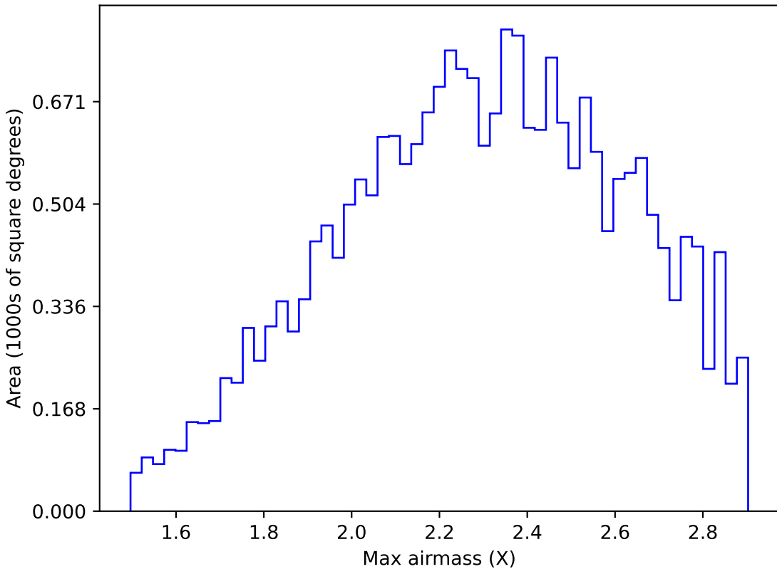
mw_roll_bulge_v3.3_10yrs All sky y band: Max airmass
