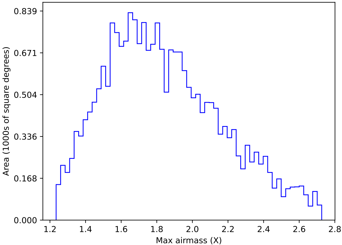
mw_roll_bulge_v3.3_10yrs All sky u band: Max airmass
