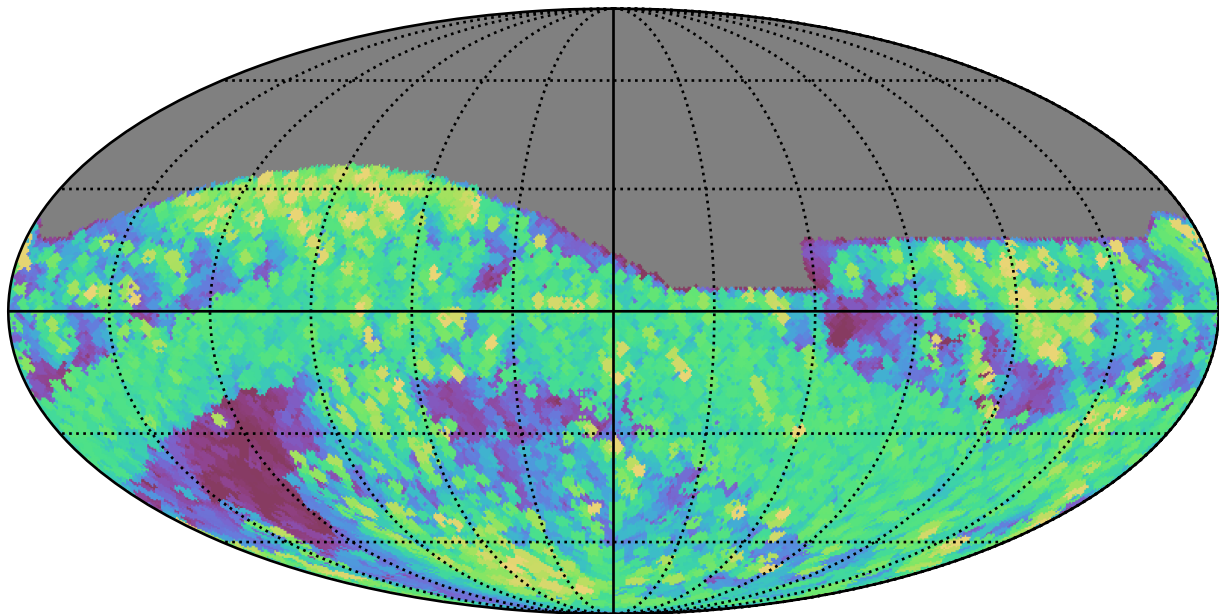
mw_roll_bulge_v3.3_10yrs All sky r band: Max airmass
