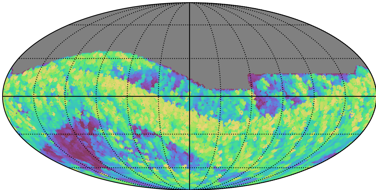
mw_roll_bulge_v3.3_10yrs All sky i band: Max airmass
