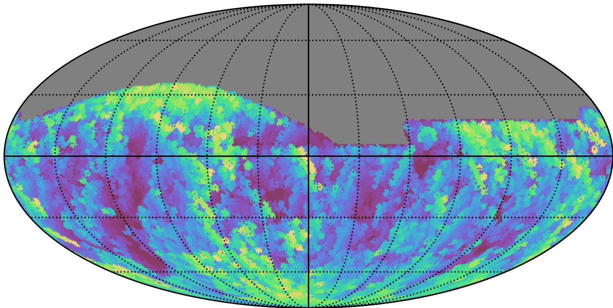
mw_roll_bulge_v3.3_10yrs All sky g band: Max airmass
