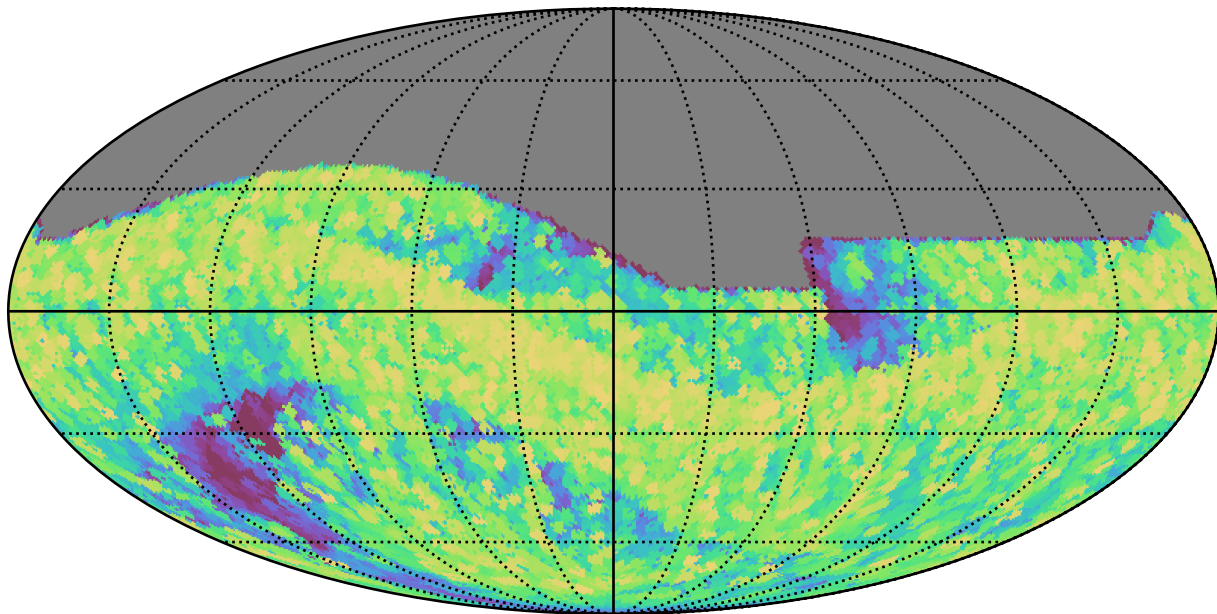
mw_roll_bulge_v3.3_10yrs All sky all bands: Max airmass
