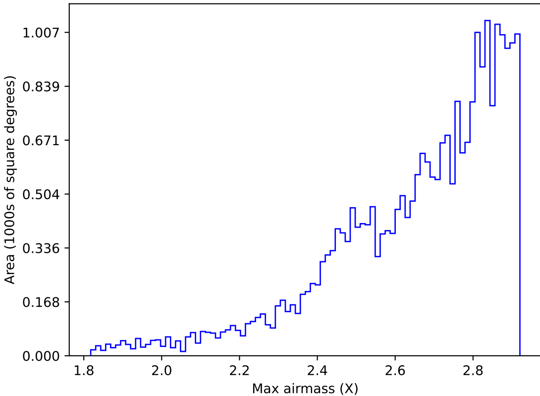
mw_roll_bulge_v3.3_10yrs All sky all bands: Max airmass
