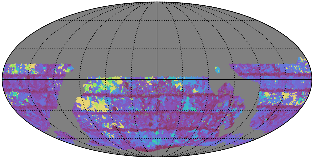
mw_roll_bulge_v3.3_10yrs WFD z band: Max Inter-Night Gap
