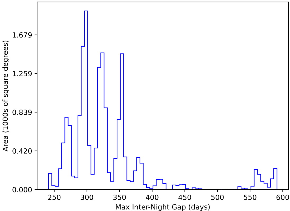
mw_roll_bulge_v3.3_10yrs WFD y band: Max Inter-Night Gap
