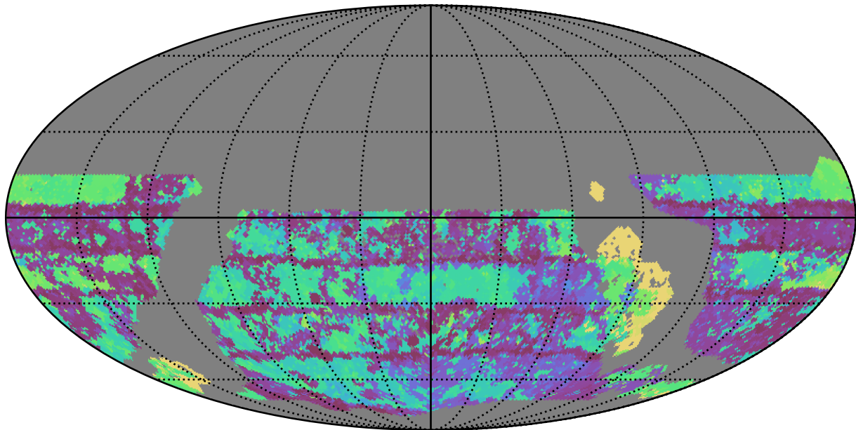
mw_roll_bulge_v3.3_10yrs WFD u band: Max Inter-Night Gap
