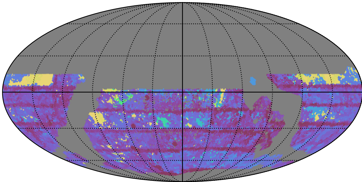
mw_roll_bulge_v3.3_10yrs WFD r band: Max Inter-Night Gap
