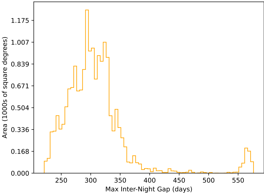
mw_roll_bulge_v3.3_10yrs WFD r band: Max Inter-Night Gap
