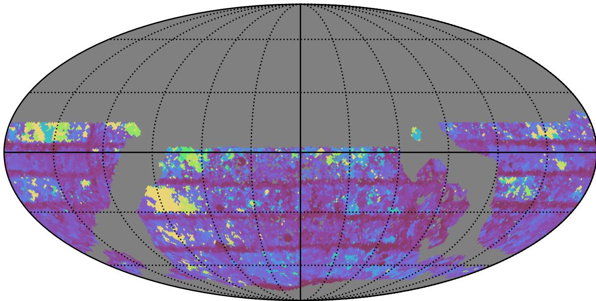
mw_roll_bulge_v3.3_10yrs WFD i band: Max Inter-Night Gap
