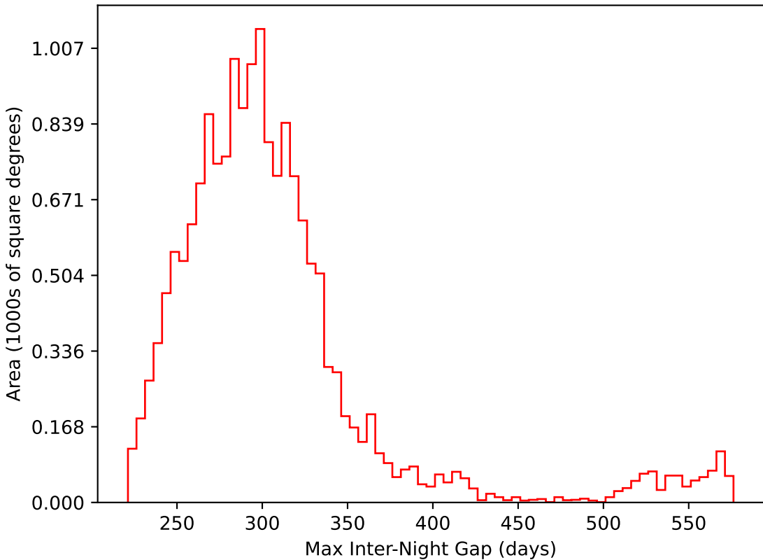
mw_roll_bulge_v3.3_10yrs WFD i band: Max Inter-Night Gap
