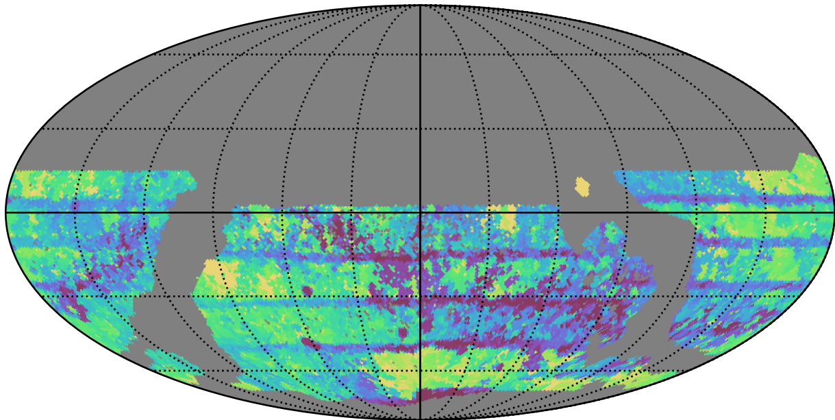
mw_roll_bulge_v3.3_10yrs WFD all bands: Max Inter-Night Gap
