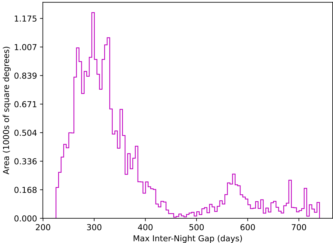
mw_roll_bulge_v3.3_10yrs All sky z band: Max Inter-Night Gap
