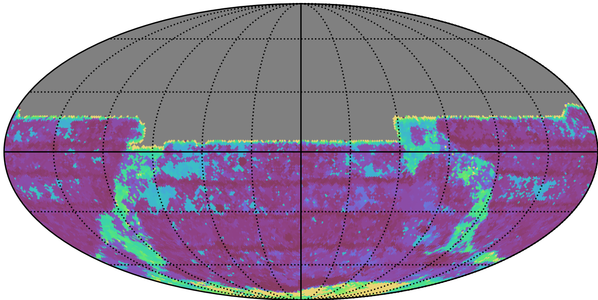
mw_roll_bulge_v3.3_10yrs All sky y band: Max Inter-Night Gap
