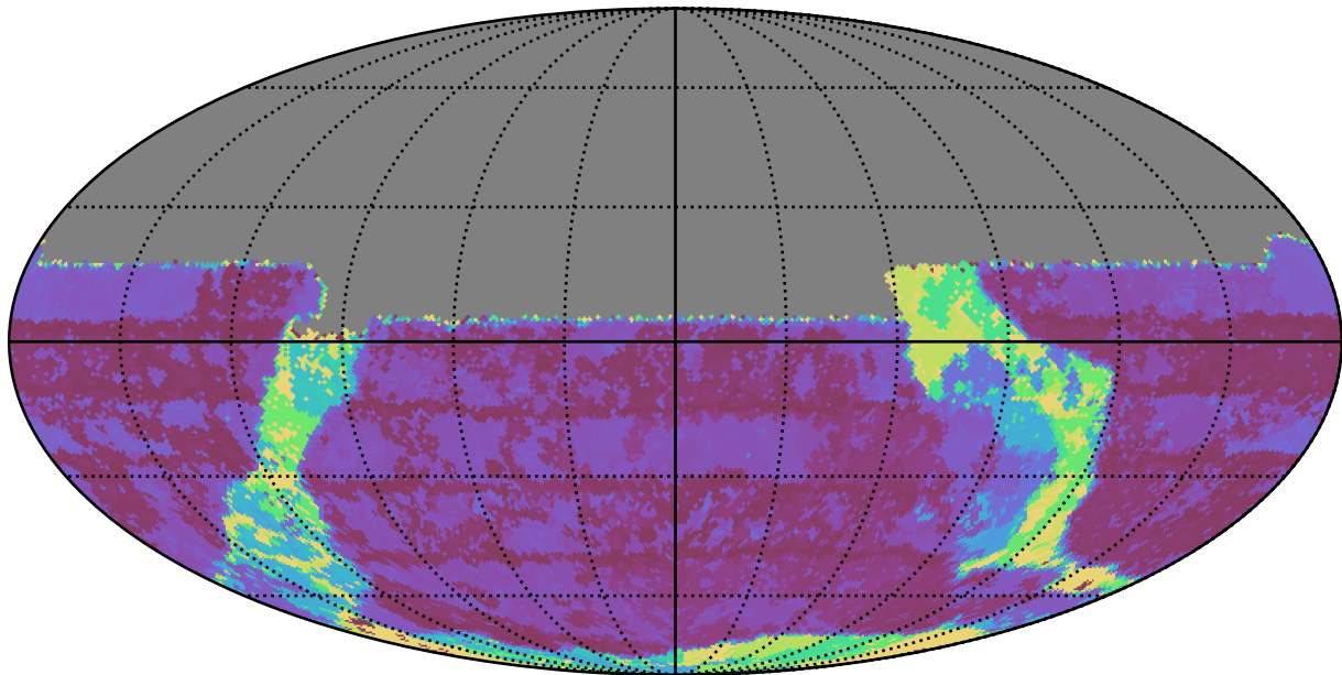
mw_roll_bulge_v3.3_10yrs All sky u band: Max Inter-Night Gap
