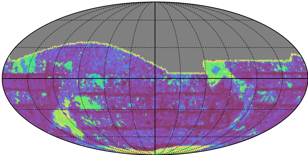
mw_roll_bulge_v3.3_10yrs All sky i band: Max Inter-Night Gap
