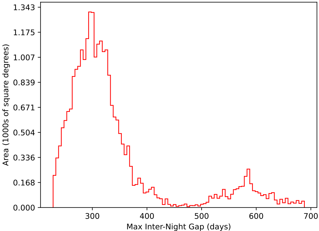
mw_roll_bulge_v3.3_10yrs All sky i band: Max Inter-Night Gap
