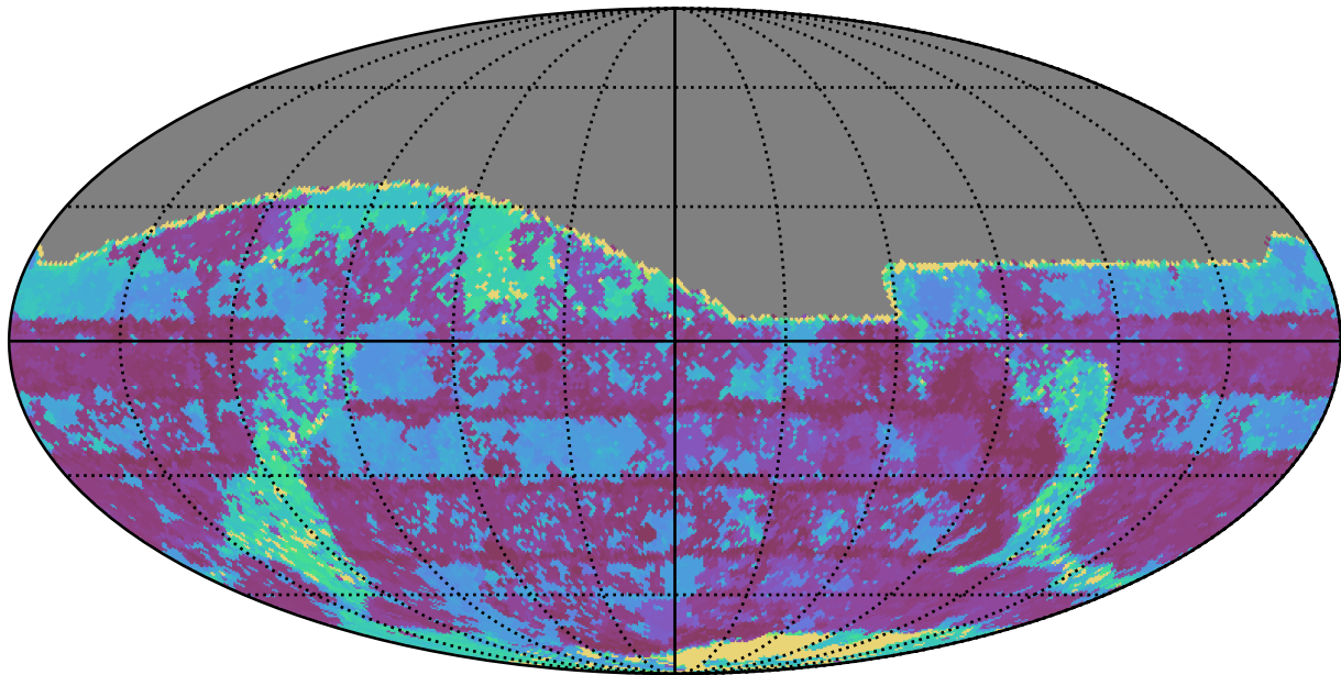
mw_roll_bulge_v3.3_10yrs All sky g band: Max Inter-Night Gap
