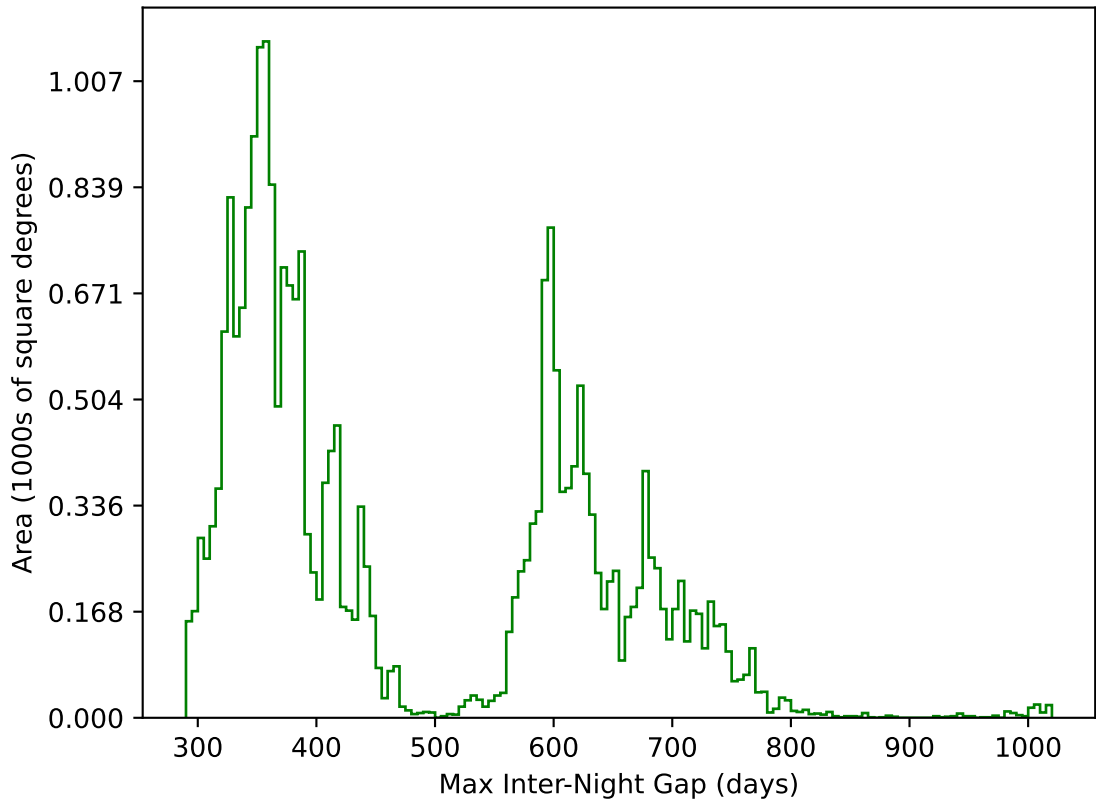
mw_roll_bulge_v3.3_10yrs All sky g band: Max Inter-Night Gap
