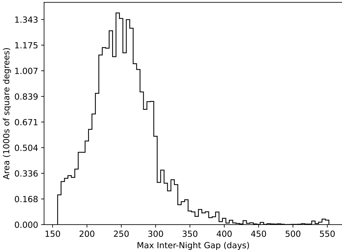
mw_roll_bulge_v3.3_10yrs All sky all bands: Max Inter-Night Gap
