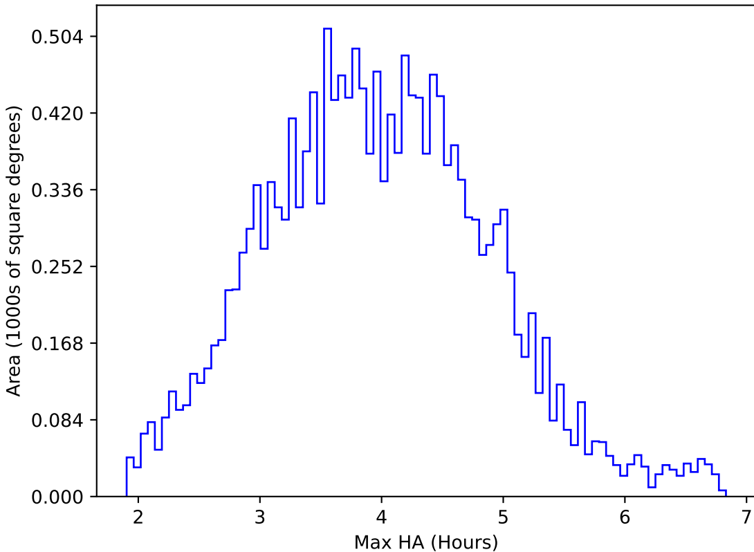
mw_roll_bulge_v3.3_10yrs WFD u band: Max HA
