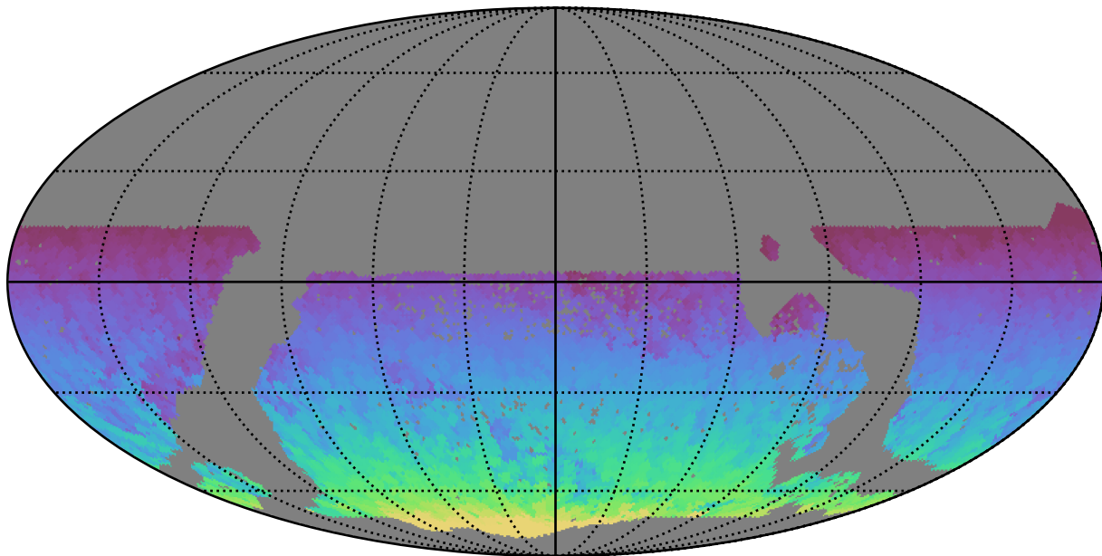
mw_roll_bulge_v3.3_10yrs WFD all bands: Max HA
