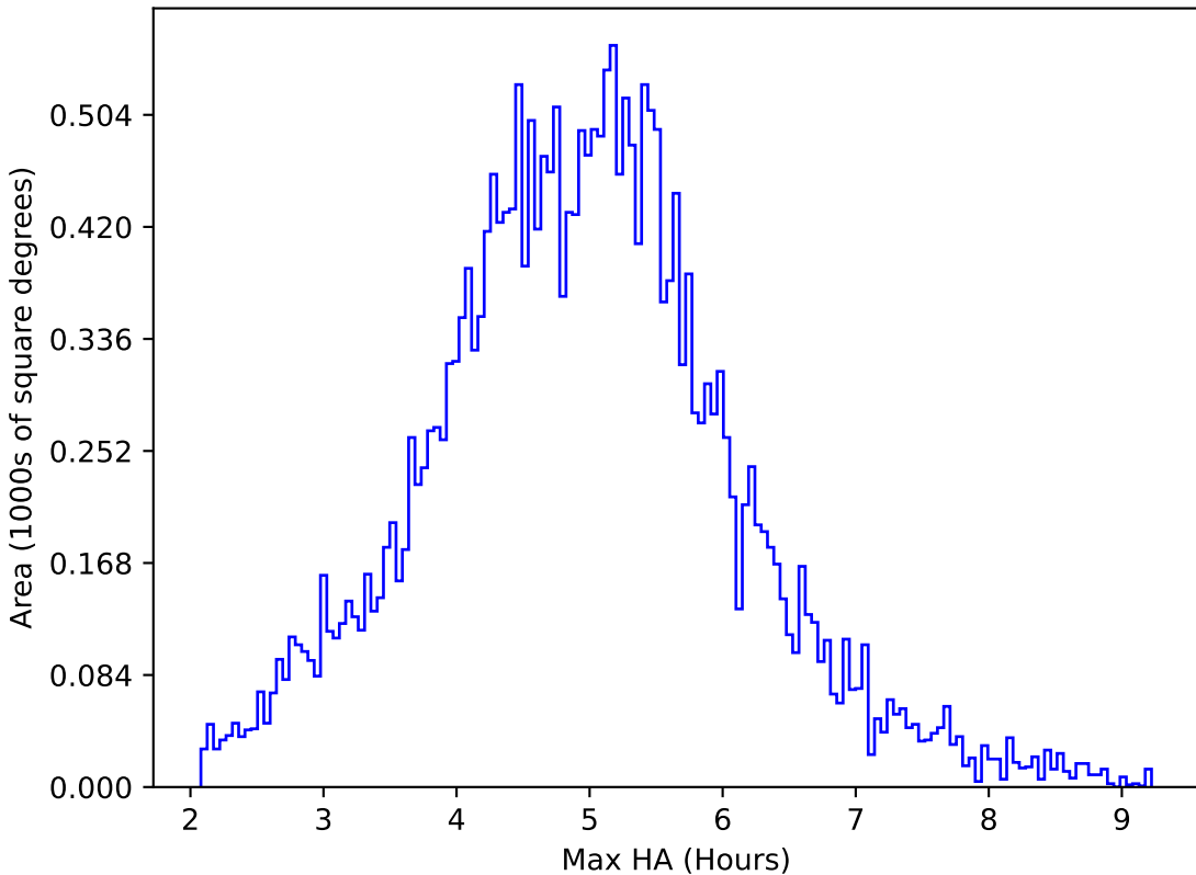
mw_roll_bulge_v3.3_10yrs All sky all bands: Max HA
