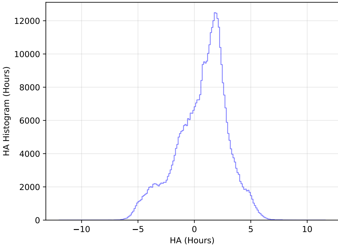
mw_roll_bulge_v3.3_10yrs WFD z band: HA Histogram
