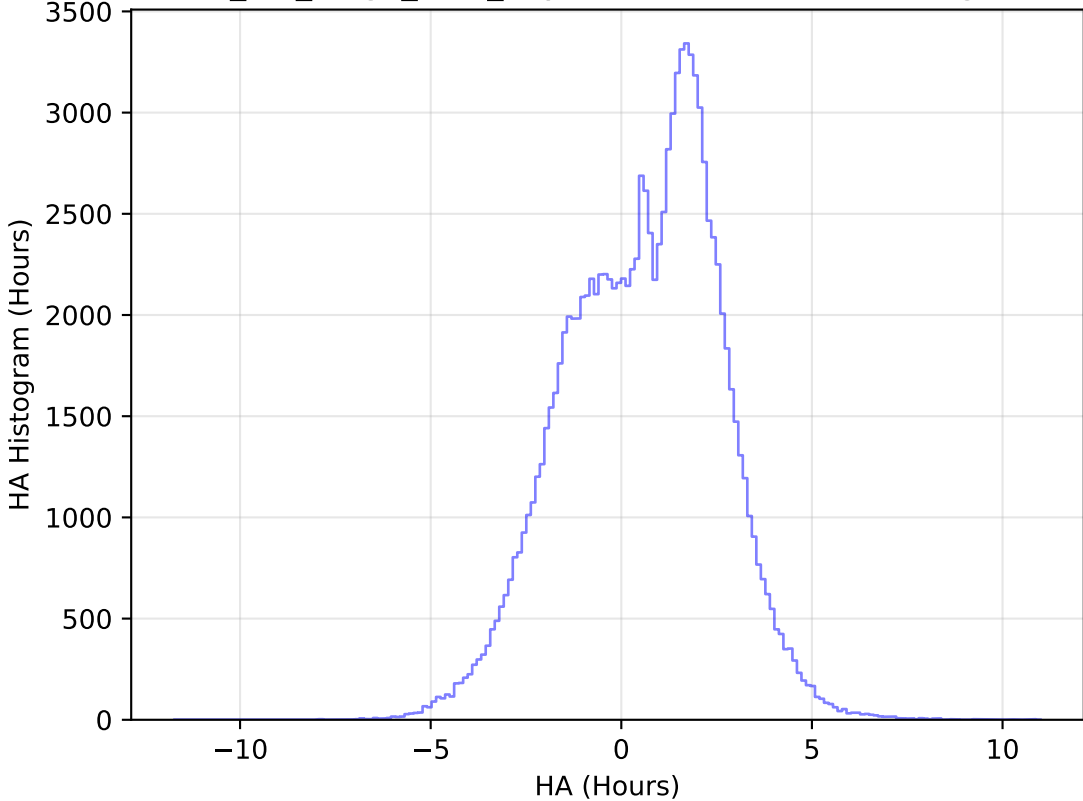
mw_roll_bulge_v3.3_10yrs WFD u band: HA Histogram
