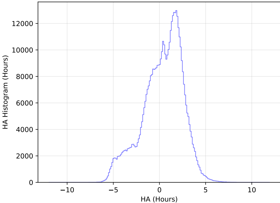
mw_roll_bulge_v3.3_10yrs WFD r band: HA Histogram
