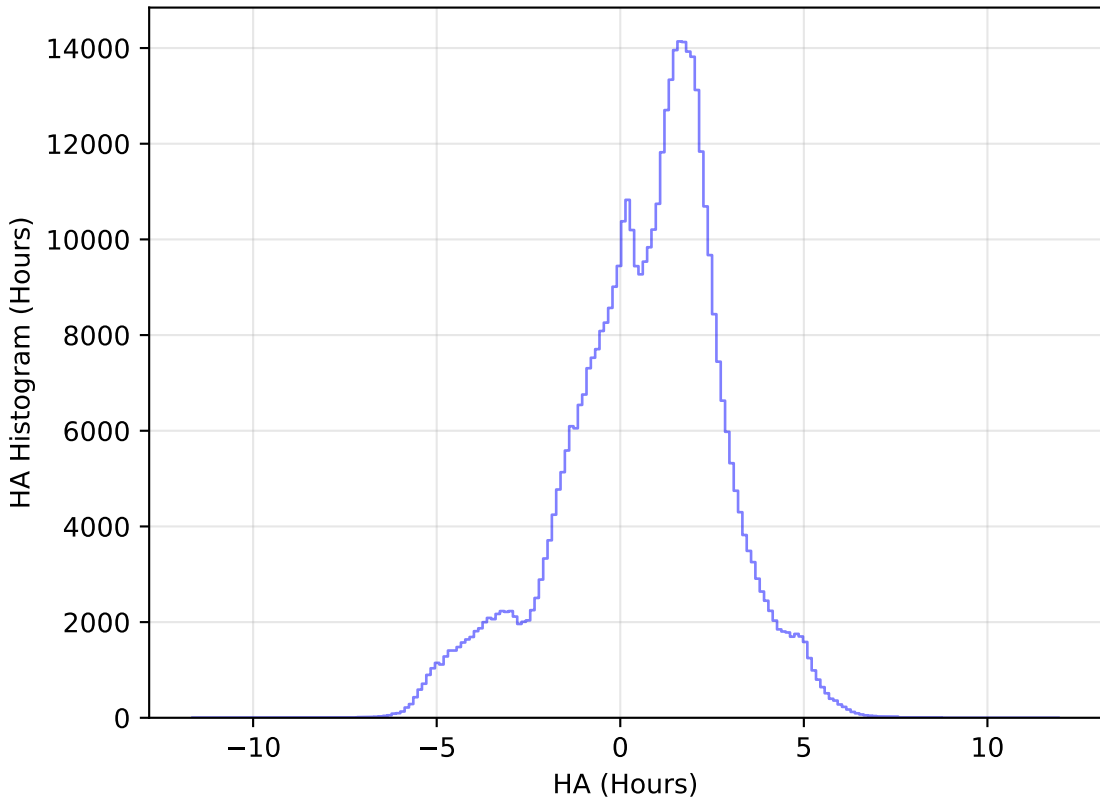
mw_roll_bulge_v3.3_10yrs WFD i band: HA Histogram
