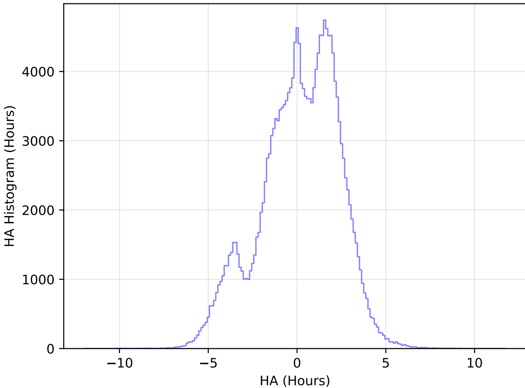
mw_roll_bulge_v3.3_10yrs WFD g band: HA Histogram
