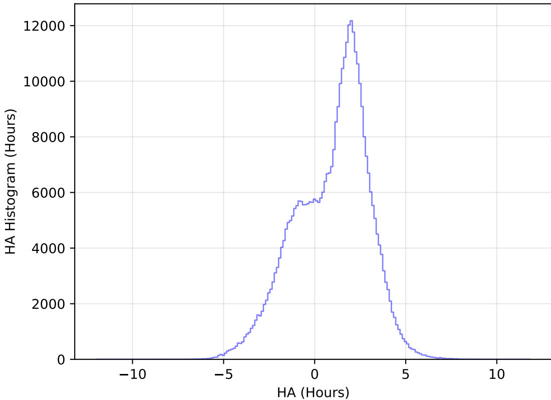
mw_roll_bulge_v3.3_10yrs All sky y band: HA Histogram
