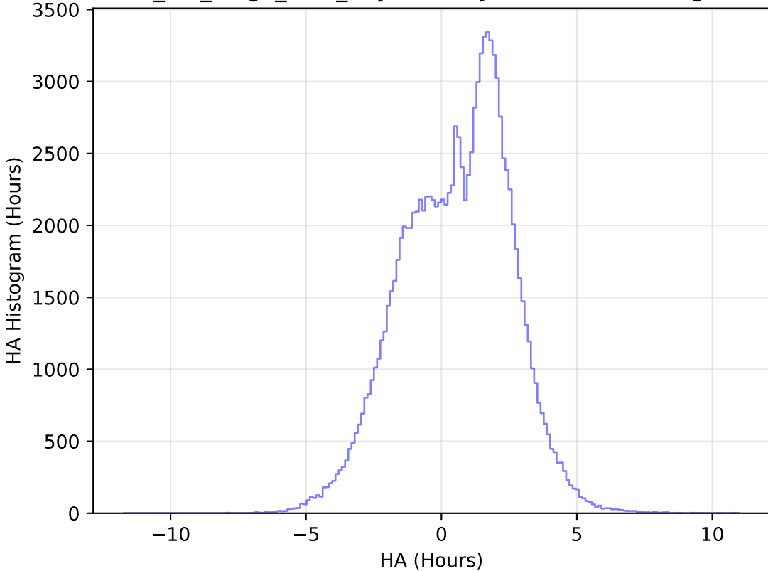
mw_roll_bulge_v3.3_10yrs All sky u band: HA Histogram
