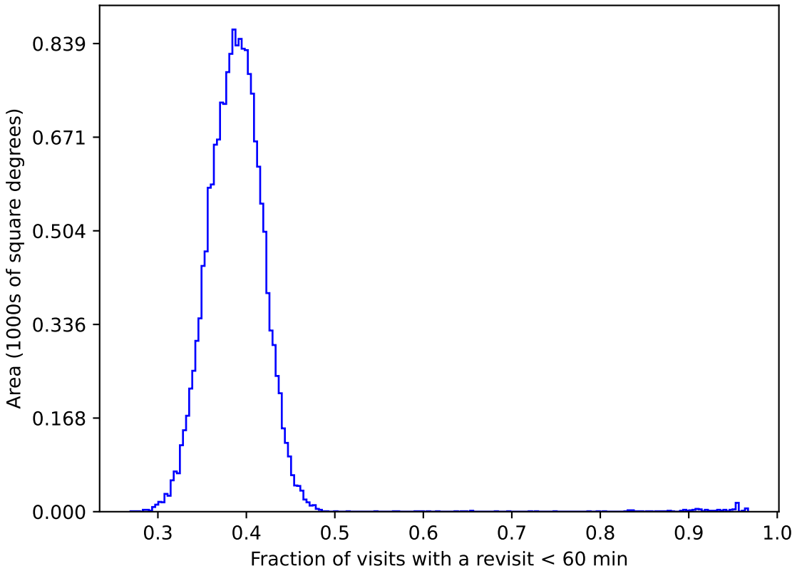
mw_roll_bulge_v3.3_10yrs gri WFD: Fraction of visits with a revisit < 60 min
