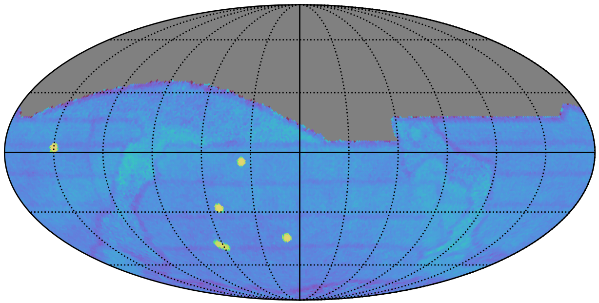
mw_roll_bulge_v3.3_10yrs gri All sky: Fraction of visits with a revisit < 60 min
