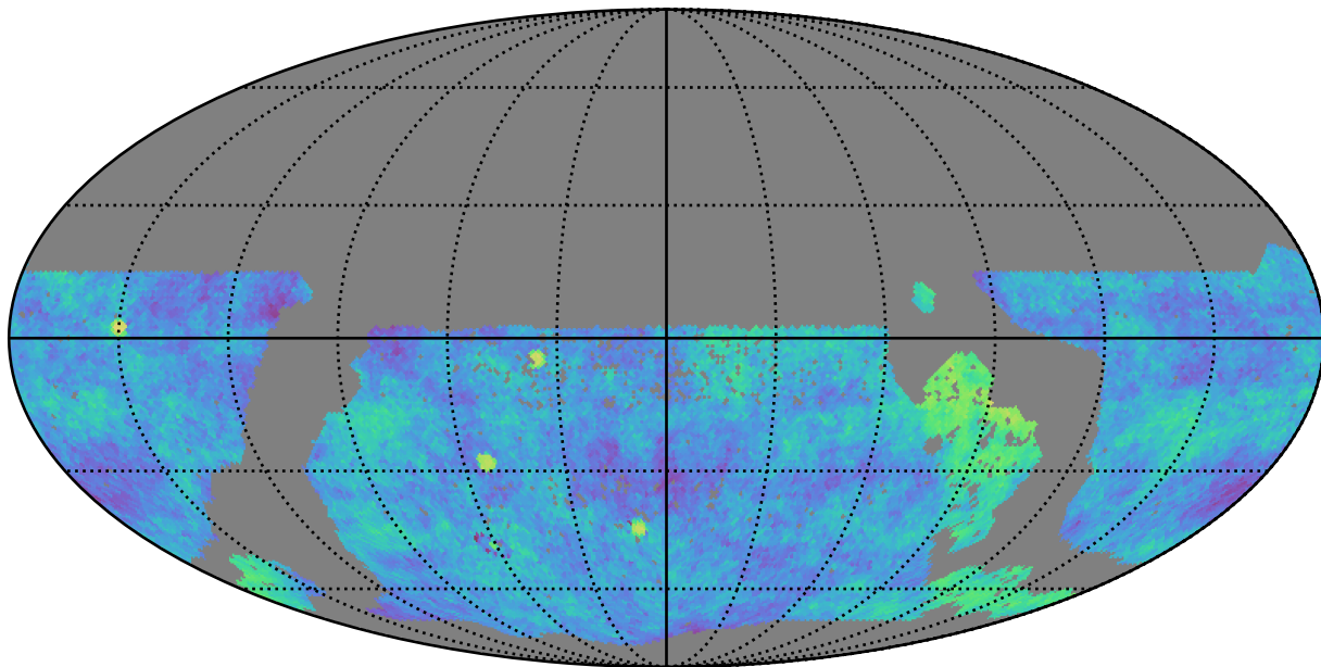
mw_roll_bulge_v3.3_10yrs gri WFD: Fraction of visits in pairs (20-90 min)
