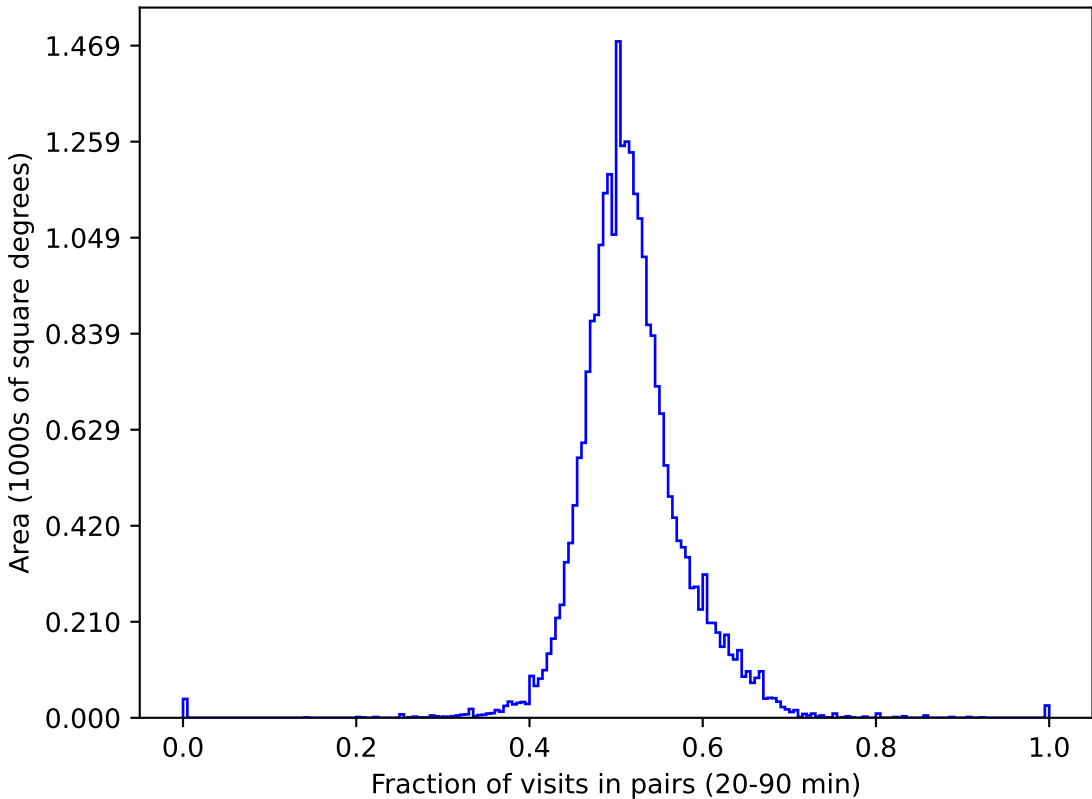
mw_roll_bulge_v3.3_10yrs gri All sky: Fraction of visits in pairs (20-90 min)
