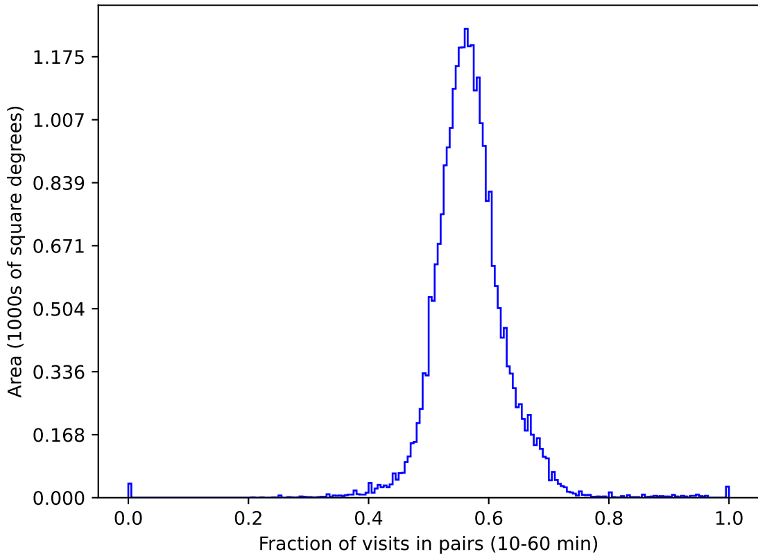
mw_roll_bulge_v3.3_10yrs gri All sky: Fraction of visits in pairs (10-60 min)
