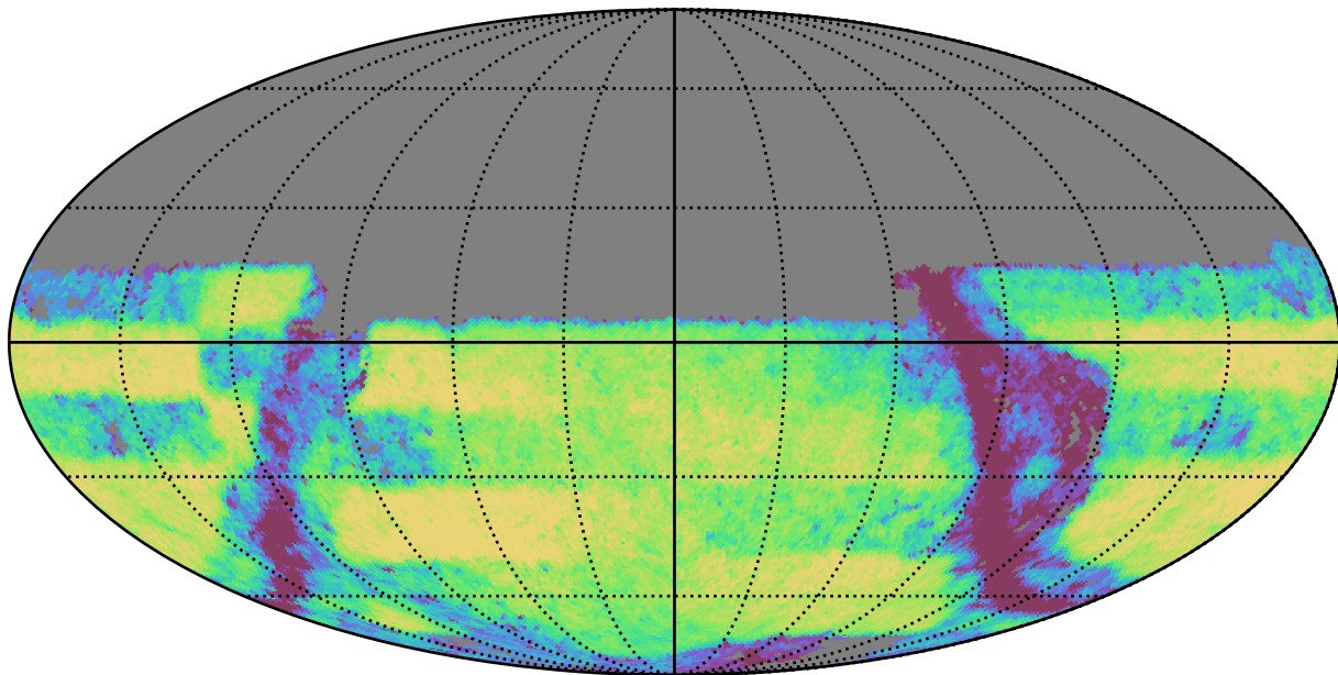
mw_roll_bulge_v3.3_10yrs Yr 3-4 y band: Exgal_CoaddM5
