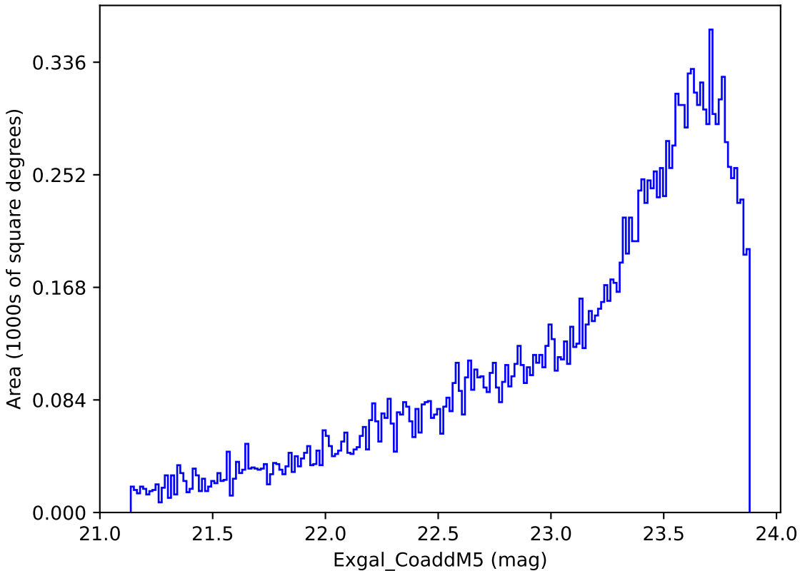
mw_roll_bulge_v3.3_10yrs Yr 3-4 y band: Exgal_CoaddM5
