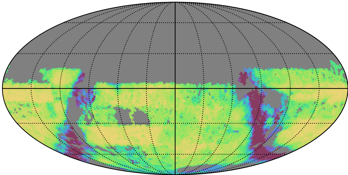
mw_roll_bulge_v3.3_10yrs Yr 3-4 u band: Exgal_CoaddM5
